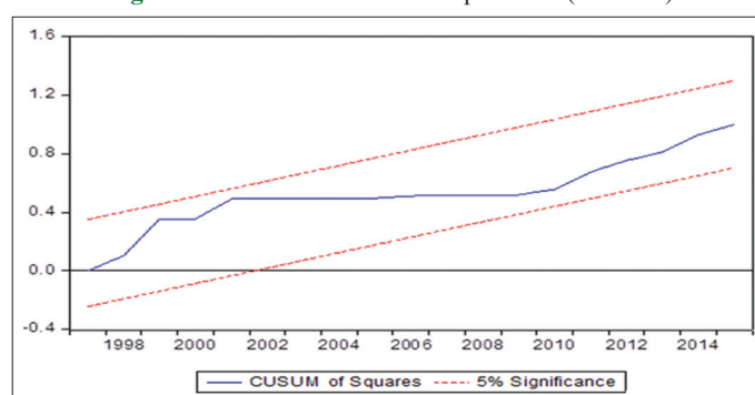
Figure 10: Results of CUSUM square test (Model 2)
