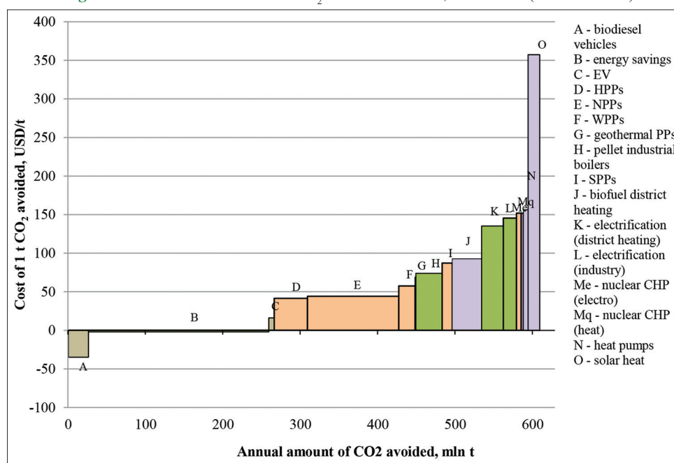
Figure 3: Total cost related to the CO 2 emission avoided, 2020-2025 (basic scenario)
