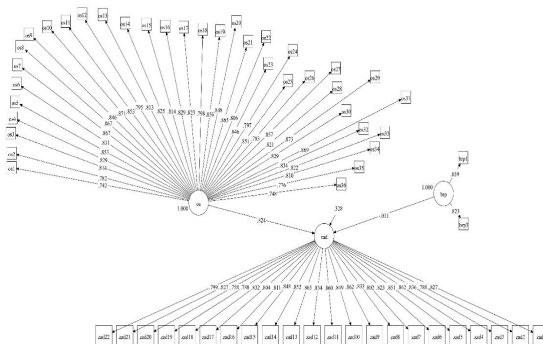
Picture 1. Path diagram with standardized coefficients
