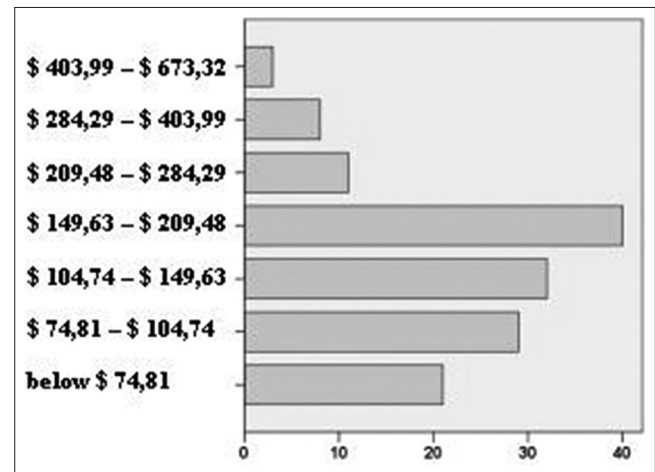
Figure 2: Distribution of respondents wishing to use solar panels to power their households, according to per capita income
