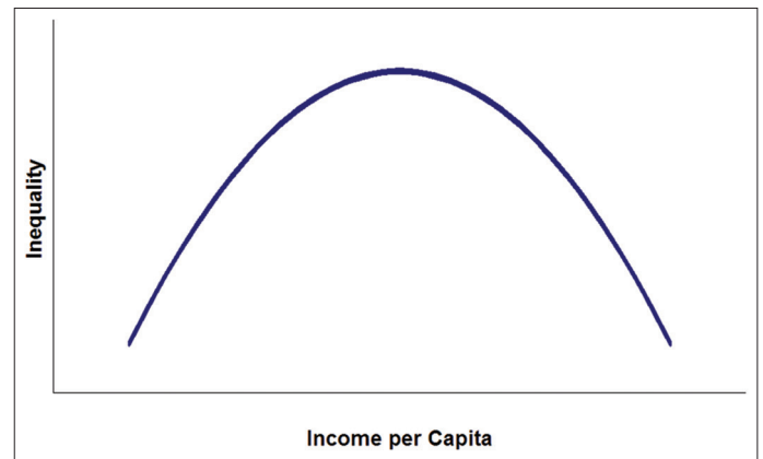
Figure 1: Kuznets' curve
