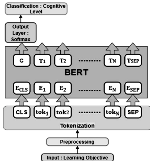
Fig. 3. BERT-based fine-tuning architecture: C – at the end; T_1, T_2, \dots, T_N – the learner, will be able, to analyze; E_{CLS} – the module; E_1, E_2, \dots, E_N – aims to equip the learner; CLS – the module's objective; tok_1, tok_2, \dots, tok_N – to enhance analytical thinking skills
