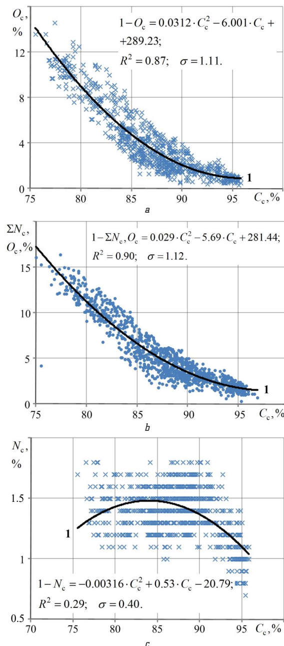
Fig. 1. Dependence of changes in the ratio of elements of coal in combustible part of the fuel: a – the ratio between the content of carbon and oxygen; b – the ratio between the content of carbon and a mixture of other components ( \Sigma N_c , O_c ); c – the ratio between the carbon content and nitrogen; 1 – averaging curves; x, o – experimental data for mine formations, respectively, according to [13] and [14]; R^2 и \sigma are, respectively, the coefficients of determination and standard deviations from the averaging curves
