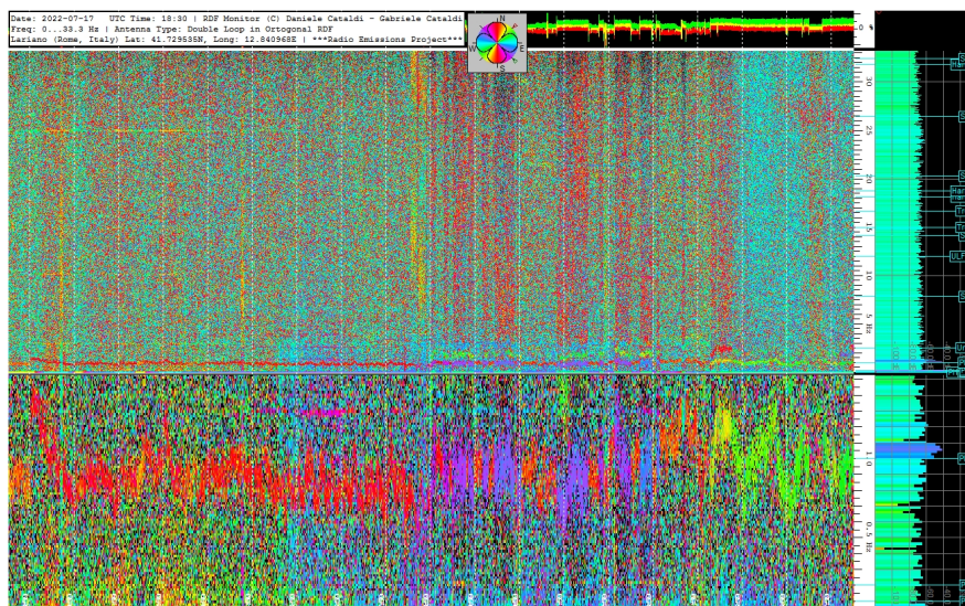
Fig. 3. Low-frequency interference whose colors indicate the azimuth of the future areal epicenter (Courtesy: Daniele Gabriele Cataldi)
