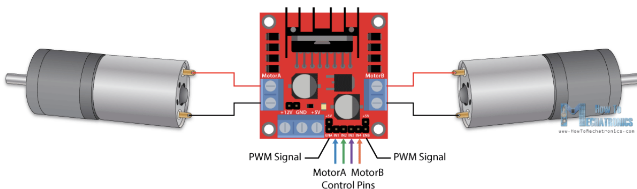
Figure 9: L298N - motor control inputs
