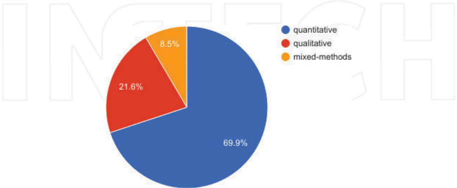
Figure 2. Research approach.
