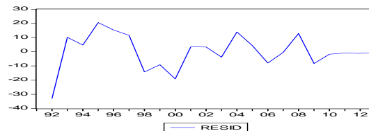
Figure 2. The variation of the residuals around zero mean
