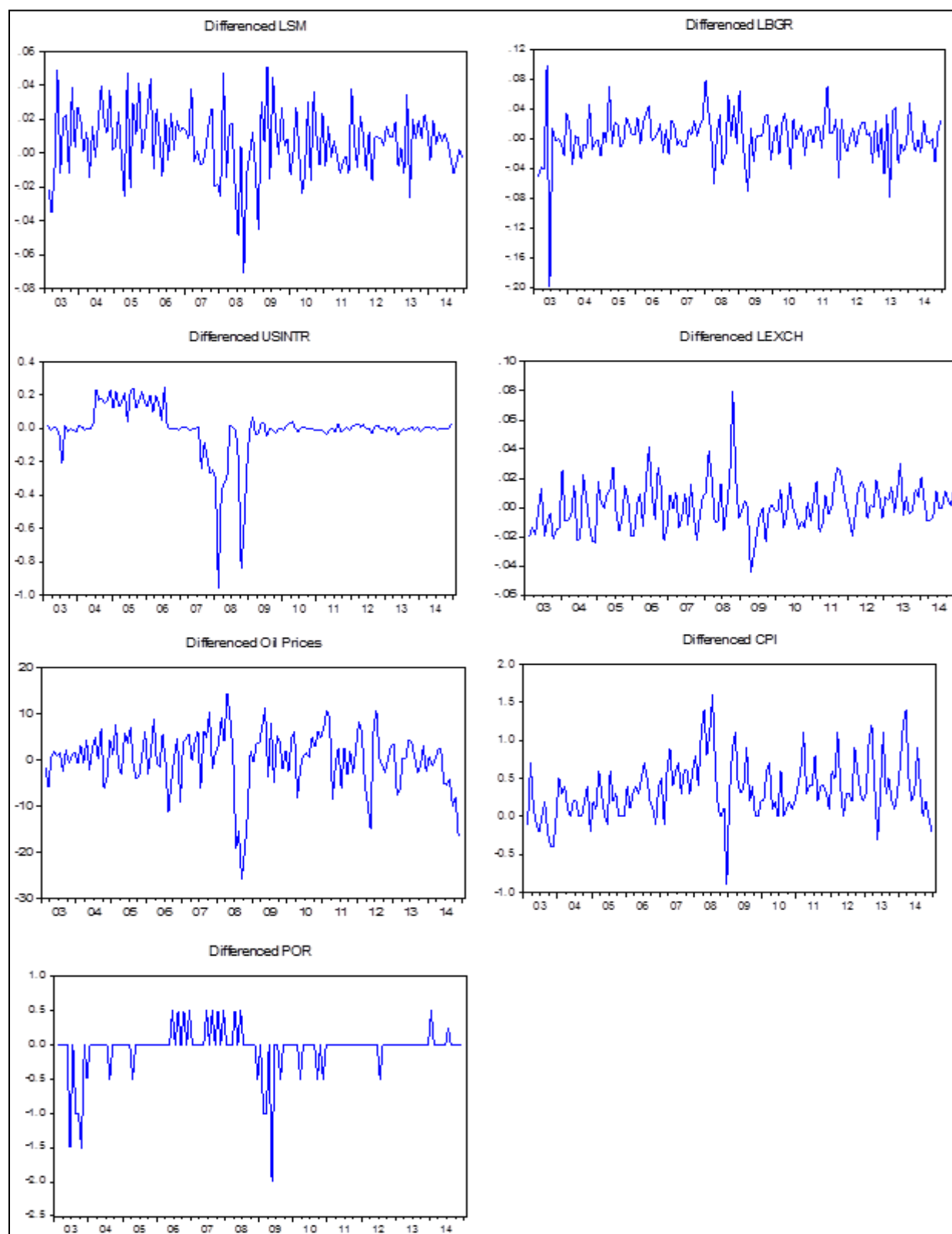
Figure 10. After-differencing graph
