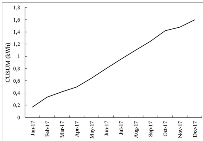
Figure 10: CUSUM graph
