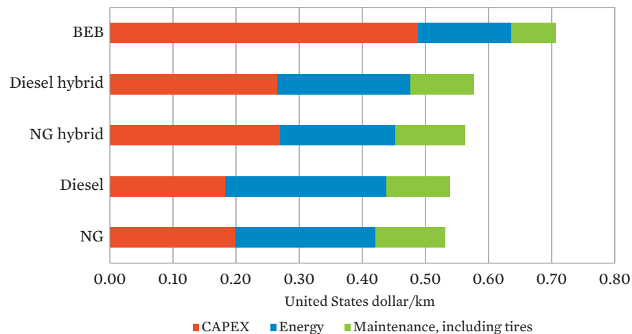
Figure 17: Total Cost of Ownership for Different Bus Technologies ($/km)
