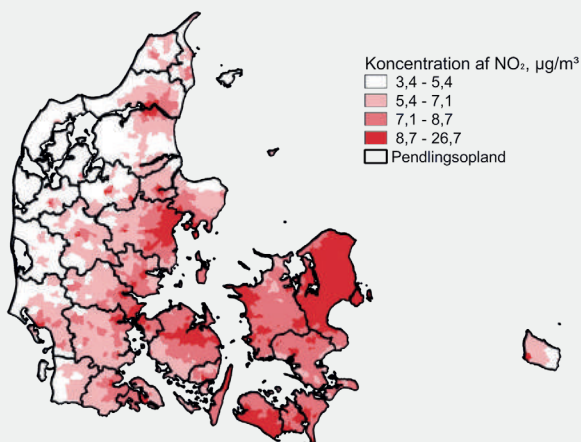
FIGUR I.2 NO 2 KONCENTRATION
