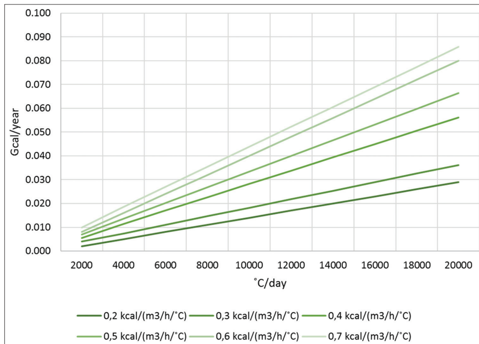
Figure 6: Thermal energy savings under various program modes of temperature change in industrial buildings ( 1/\text{m}^3 )
