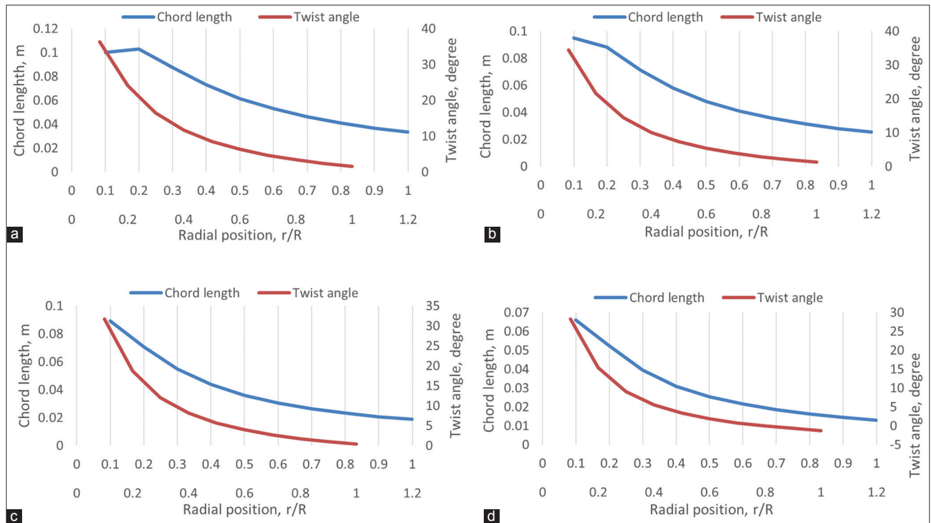
Figure 8: (a) Chord and twist distribution for SWT_re0.2 turbine. (b) Chord and twist distribution for SWT_re0.25 turbine. (c) - Chord and twist distribution for SWT_re0.3 turbine. (d) Chord and twist distribution for SWT_re0.35 turbine
