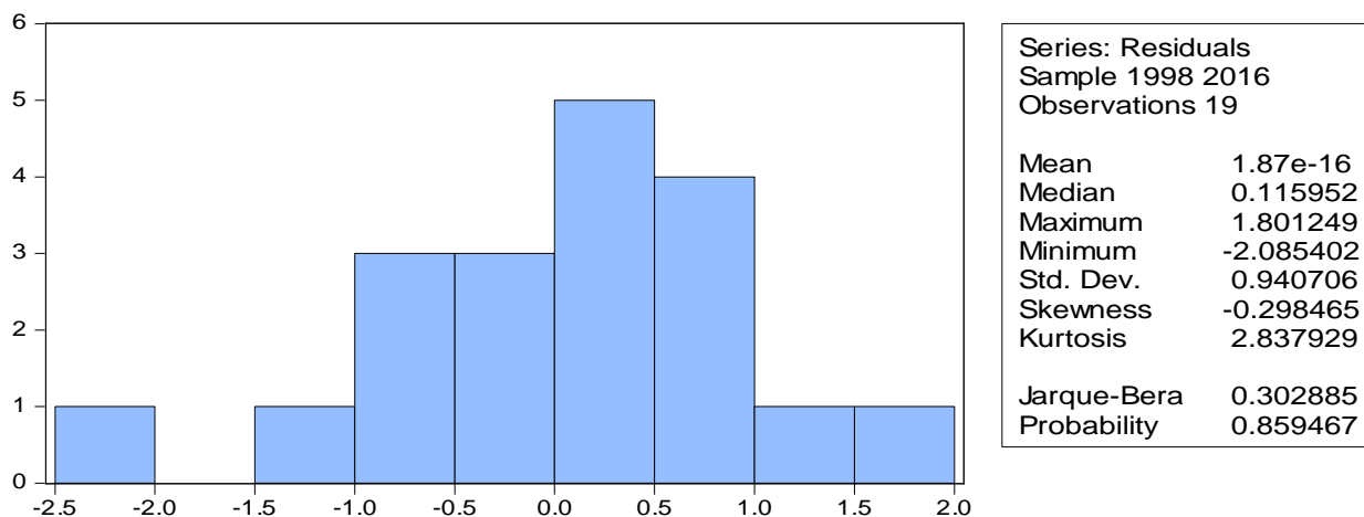
Fig. 3: Normality Test
