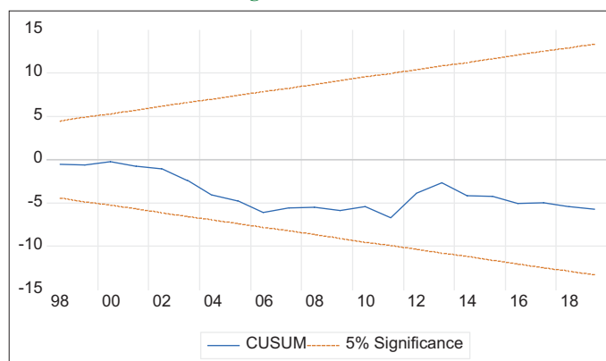
Figure 4: CUSUM
