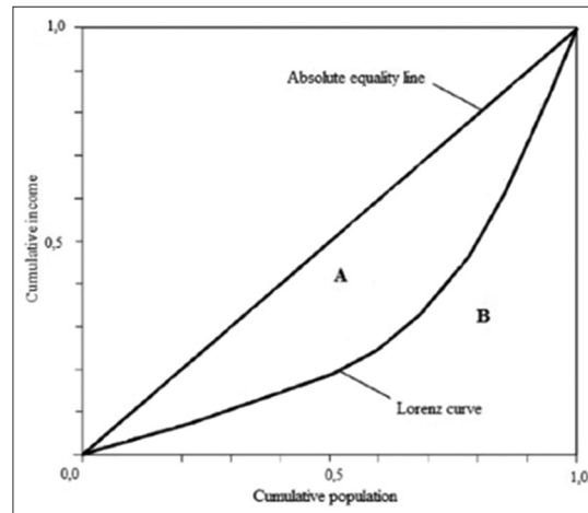
Figure 1: Lorenz Curve
