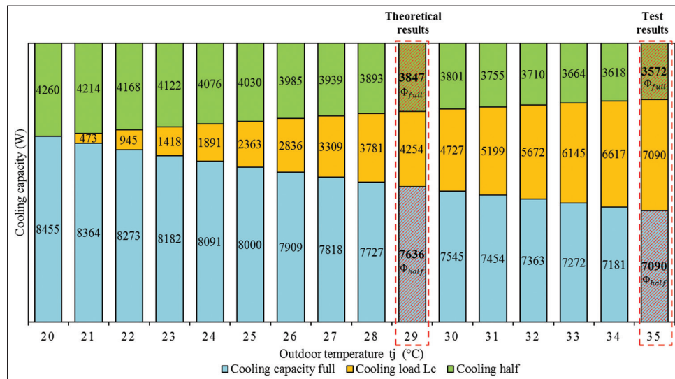
Figure 2: Cooling capacity evaluated at different outdoor temperature. Test result of ISO 16358-1
