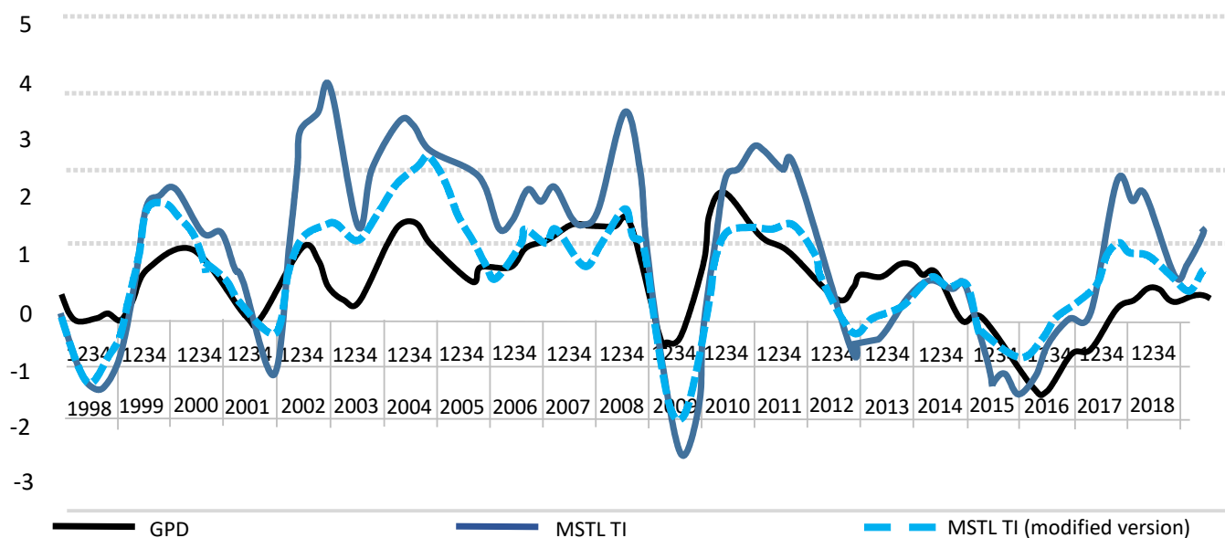
Figure 2. Moving averages of the GDP growth rate and of the traditional and modified versions of MSTL by IT classification
