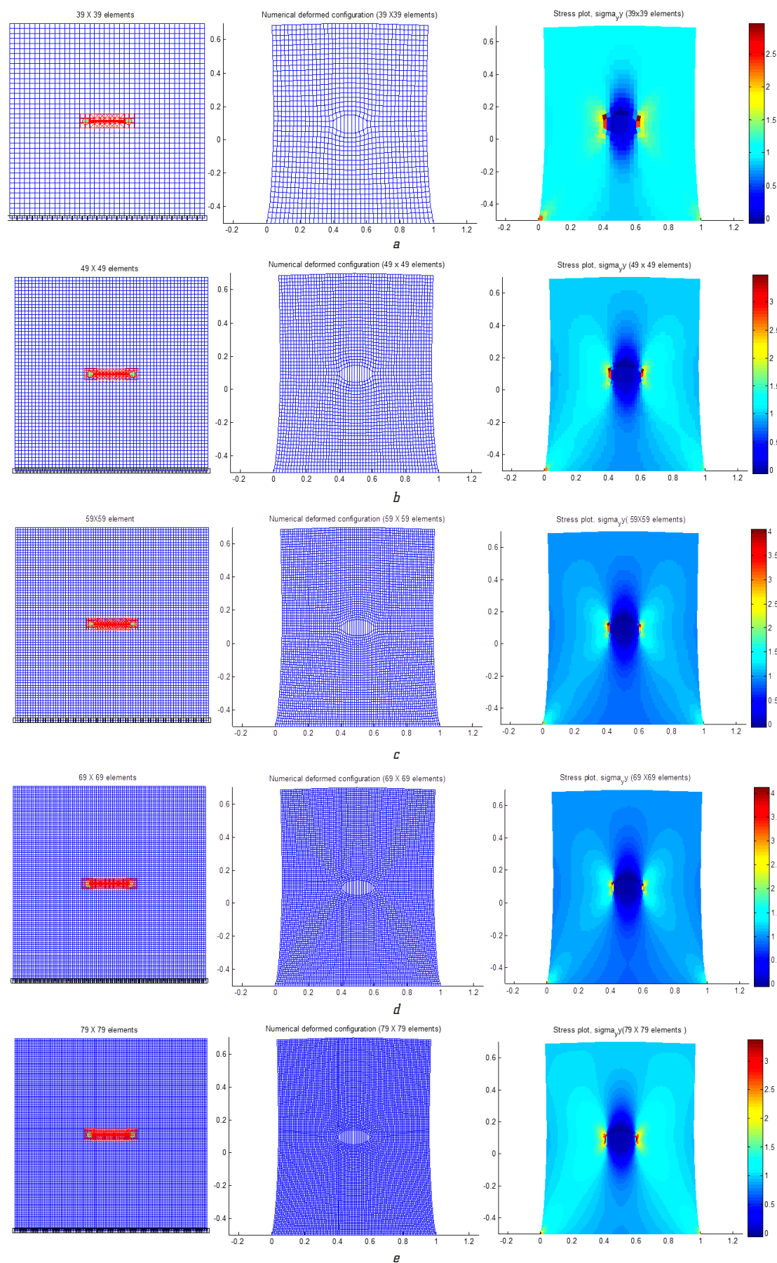
Fig. 4. Stress and deformed configuration results for different mesh refinement: a – cracked plate model result with 39 \times 39 elements; b – cracked plate model result with 49 \times 49 elements; c – cracked plate model result with 59 \times 59 elements; d – cracked plate model result with 69 \times 69 elements; e – cracked plate model result with 79 \times 79 elements
