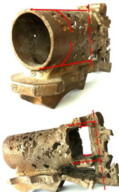
Fig. 1. Defective casting with uncult gating system
