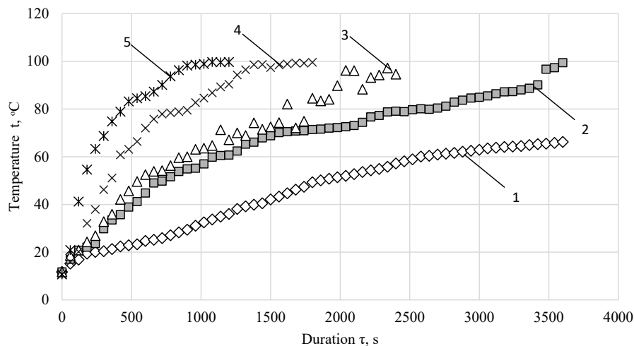
Fig. 3. The influence of the level of the supplied power of IR radiation on the change in the temperature of the product over time: 1 – 1.9 \text{ kW/m}^2 ; 2 – 3.8 \text{ kW/m}^2 ; 3 – 6 \text{ kW/m}^2 ; 4 – 8.8 \text{ kW/m}^2 ; 5 – 11.3 \text{ kW/m}^2
