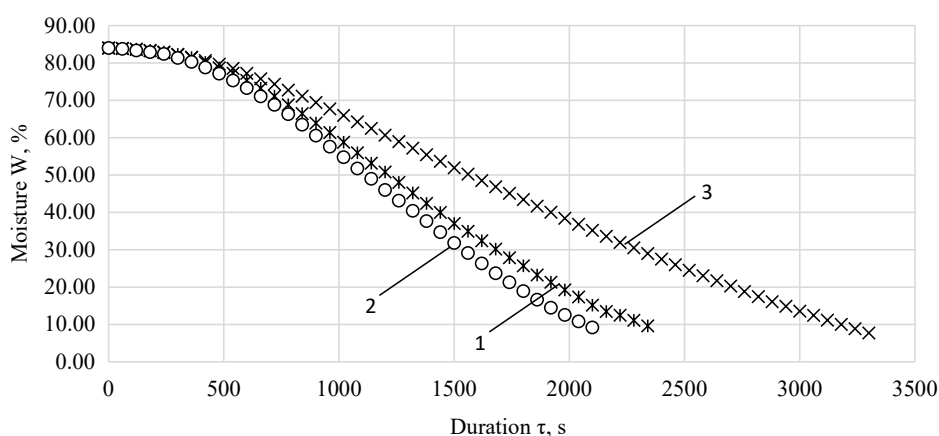
Fig. 6. Changes in moisture content of slices of vegetables and fruits over time: 1 – carrot; 2 – apple; 3 – onion
