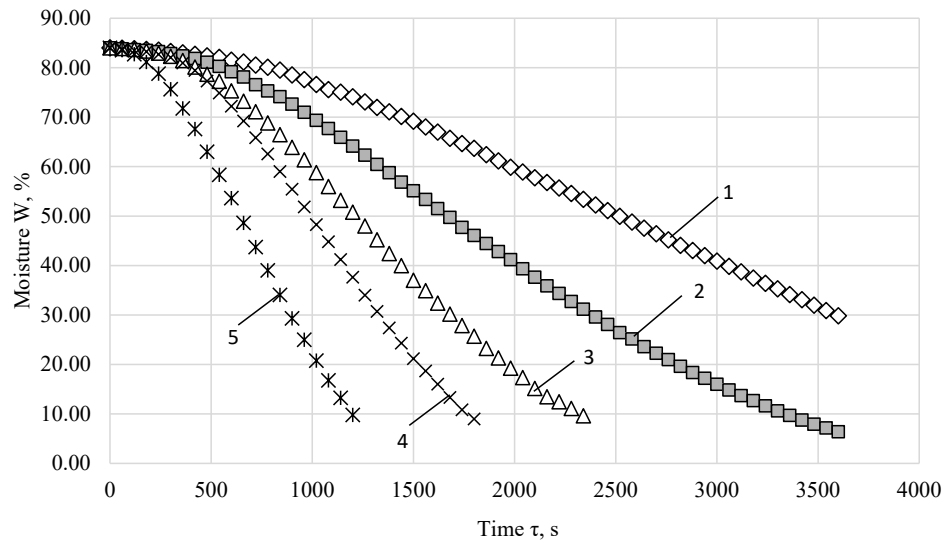
Fig. 2. The influence of the level of the supplied power of IR radiation on the change in product moisture content over time: 1 – 1.9 \text{ kW/m}^2 ; 2 – 3.8 \text{ kW/m}^2 ; 3 – 6 \text{ kW/m}^2 ; 4 – 8.8 \text{ kW/m}^2 ; 5 – 11.3 \text{ kW/m}^2
