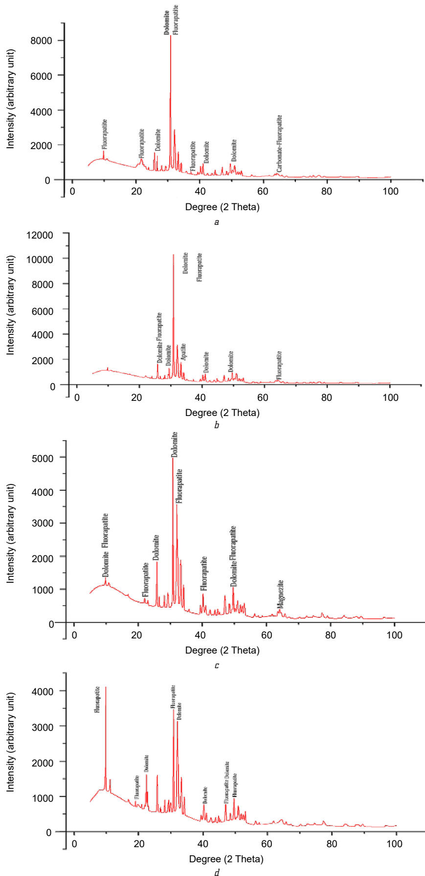
Fig. 7. XRD samples (a – waste +15 mm, Np; b – waste +15 mm, Sp; c – waste +1, +2 mm, Np; d – mud)
