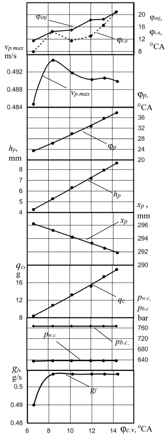
Fig. 3. Load characteristics of the 50RT-flex common rail fuel supply system
