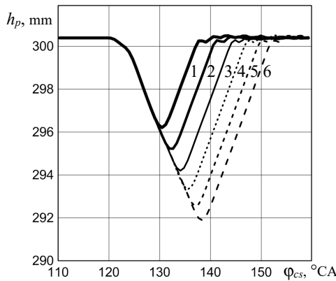
Fig. 2. Dependence of the stroke metering piston on the angle of rotation the crankshaft: 1 – \varphi_v=6.6 °CA; 2 – \varphi_v=8.4 °CA; 3 – \varphi_v=10.2 °CA; 4 – \varphi_v=12 °CA; 5 – \varphi_v=13.2 °CA; 6 – \varphi_v=14.4 °CA
