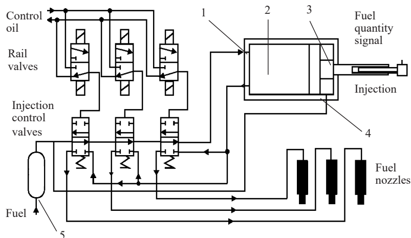
Fig. 1. Accumulator fuel injection system CRS of RT-flex engines:
