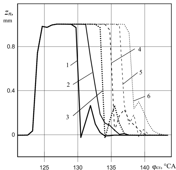
Fig. 6. Movement of the nozzle needle at different angles of opening the control valve: 1 – \varphi_v=6.6 °CA; 2 – \varphi_v=8.4 °CA; 3 – \varphi_v=10.2 °CA; 4 – \varphi_v=12 °CA; 5 – \varphi_v=13.2 °CA; 6 – \varphi_v=14.4 °CA
