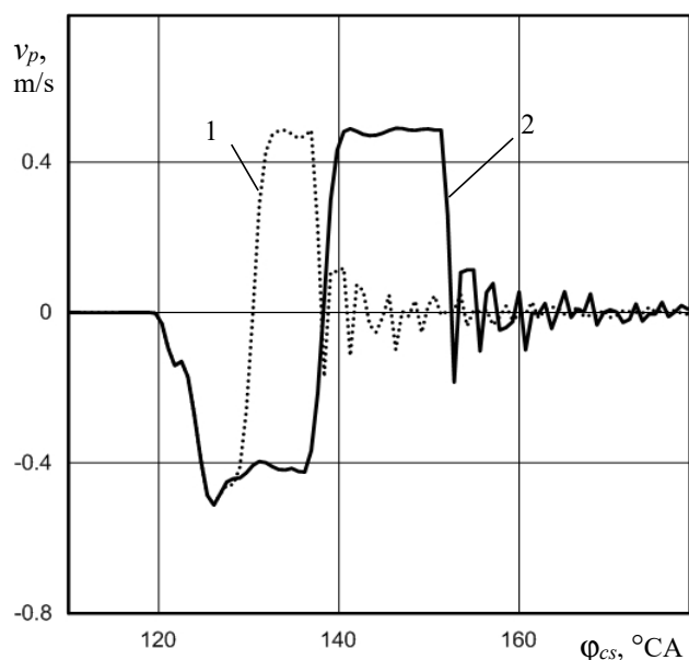
Fig. 4. Graphs of DP speeds for extreme values \varphi_v : 1 – 6.6 °CA; 2 – 14.4 °CA
