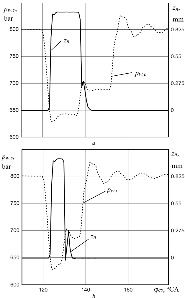
Fig. 5. Oscillograms of injector operation at: a – \varphi_v=14.4 °CA; b – \varphi_v=6.6 °CA; z_n – stroke of the nozzle needle; p_{w.c} – pressure in the working cavity of the ICU
