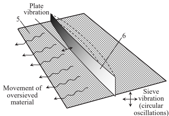
Fig. 2. Illustration of the vibrational movement of the elastic plate over the sieve – the active working body
