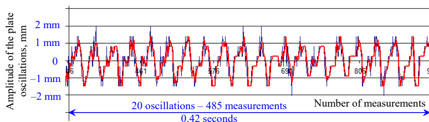
Fig. 10. Plate oscillation diagram (tensor resistor 8); working mode
