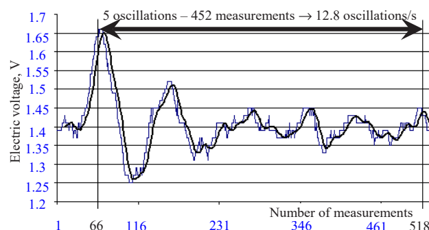
Fig. 7. Diagram of natural oscillations of the vibrating table (strain resistor 16 in Fig. 3)
