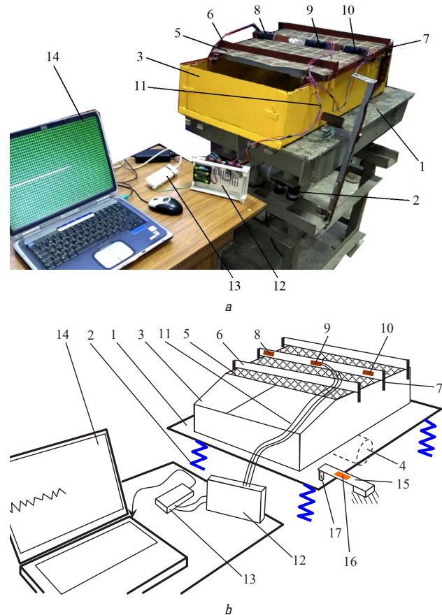
Fig. 3. Experimental setup for studying the vibrosieve:
