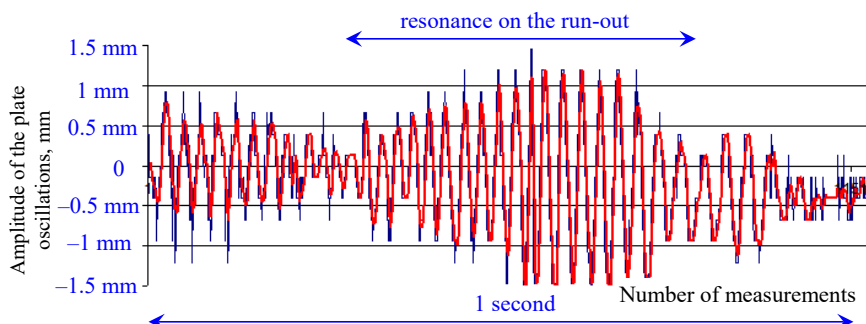
Fig. 11. Diagram of the plate oscillations (tensor resistor 9) near resonance
