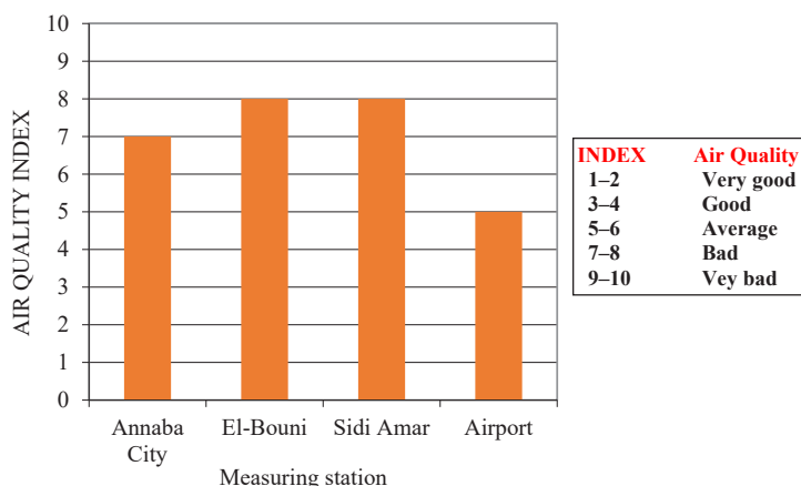
Fig. 12. Air quality index (AQI) in Annaba province
