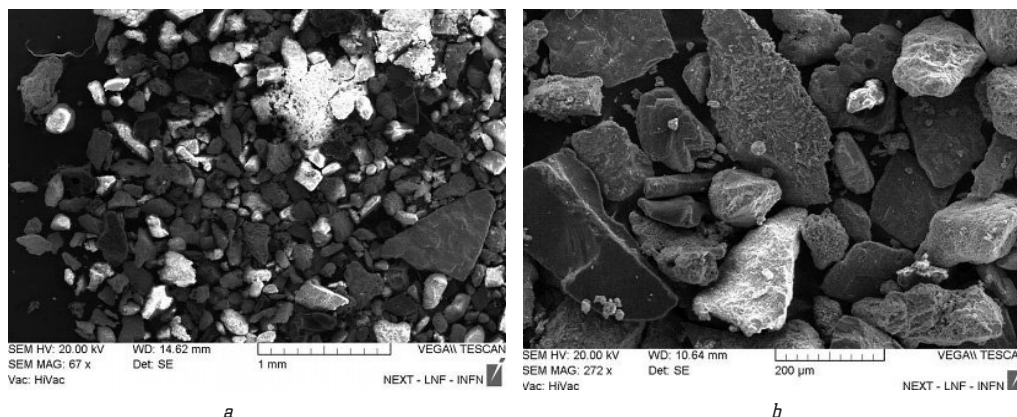
Fig. 4. Two different magnifications of the particles present in the dust DC1: a – magnification of 1 mm; b – magnification of 200 \mu\text{m}
