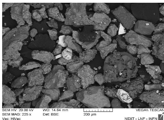
Fig. 8. BSE detector image of the sample DC2
