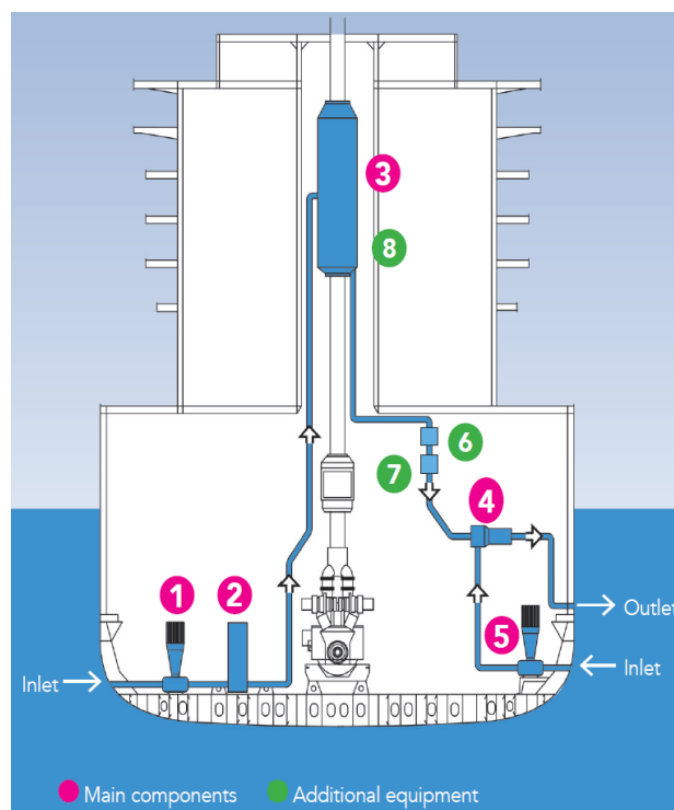
Fig. 2. Completion of the ship exhaust gas purification system:
