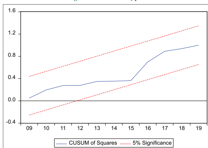
Figure 4: CUSUMSQ plot
