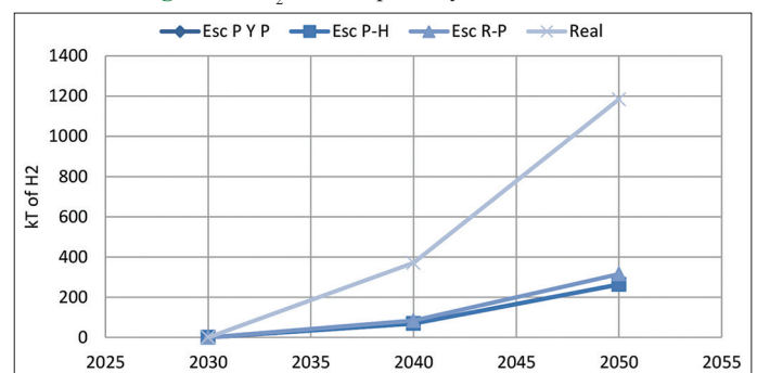
Figure 11: H 2 Consumption by scenarios in kT
