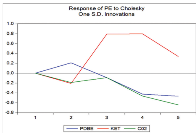
Figure 4: Impulse response function
