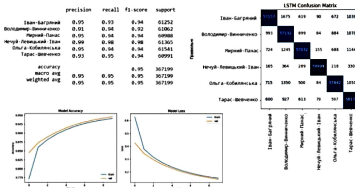
Fig. 1. Results of LSTM training period in 10 epochs
