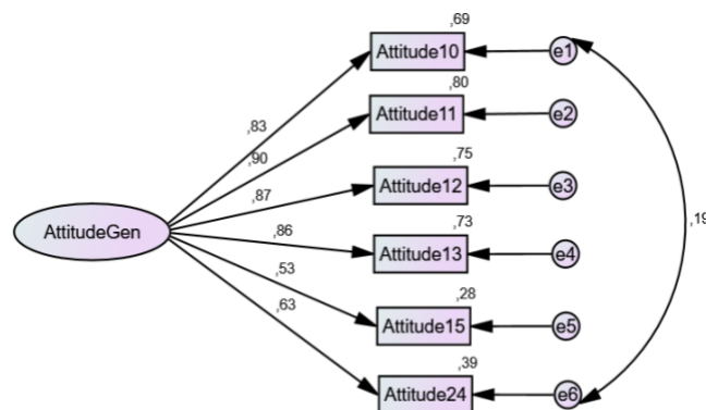
Figure 3. Exploratory Factor Analysis
