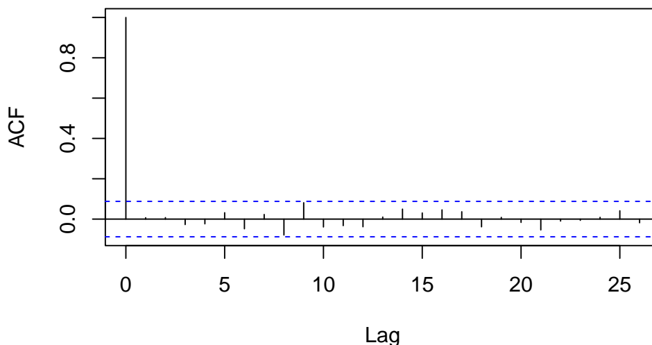
Series adl21_dynamic$residuals
