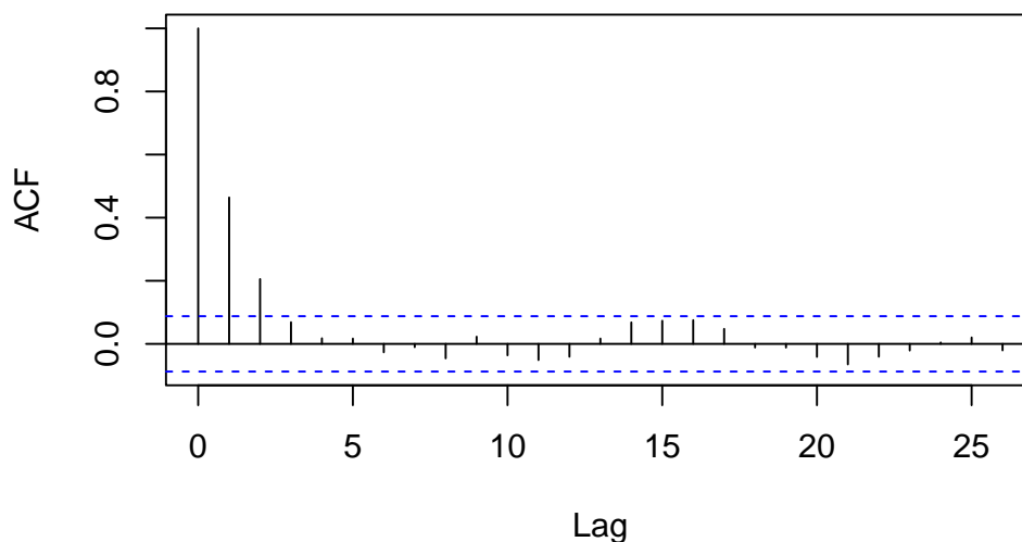
Series residuals(dlm)
