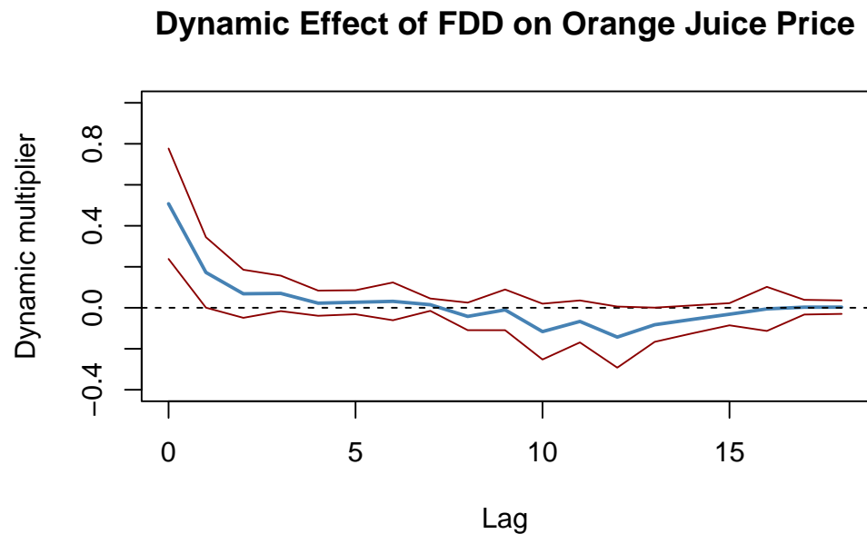
Figure 15.1: Dynamic Multipliers
