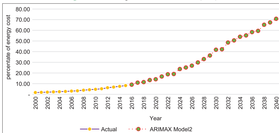
Figure 5: Forecasting from ARIMAX model 2 (2,1,2)
