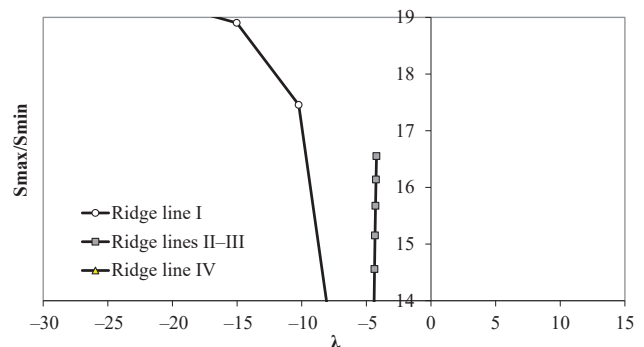
Fig. 5. Function y=\gamma(\lambda) in case of choosing the monthly period of funds allocation x_3=0
