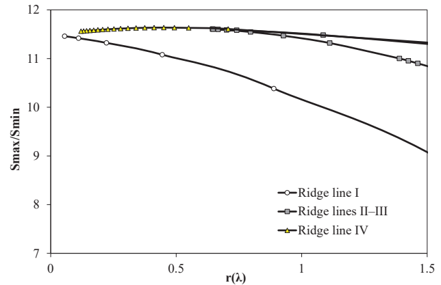
Fig. 3. Function y=\gamma(r) in case of choosing a monthly period of funds allocation x_3=-1
