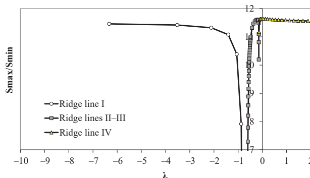
Fig. 11. Function y=y(\lambda) in the case of choosing a quarterly period of funds allocation for x_3=-1
