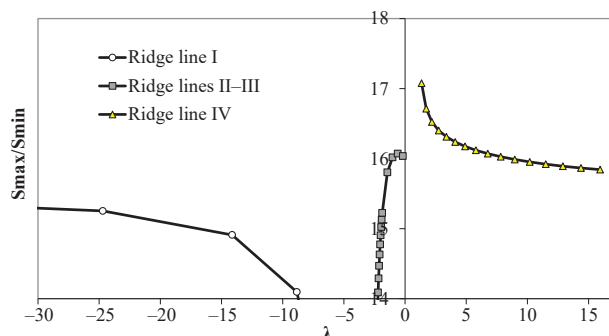
Fig. 8. Function y=y(\lambda) in the case of choosing a monthly period of funds allocation x_3=+1
