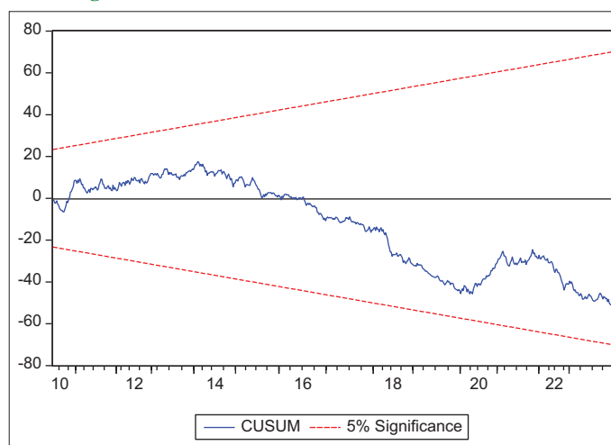
Figure 1: Plots of cumulative sum of recursive residuals
