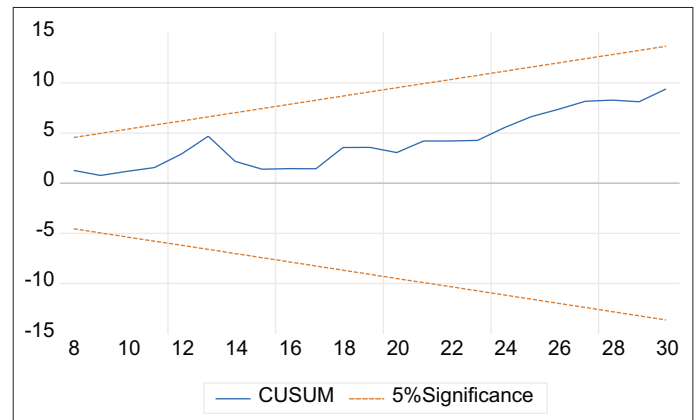
Figure 1: Cusum test
