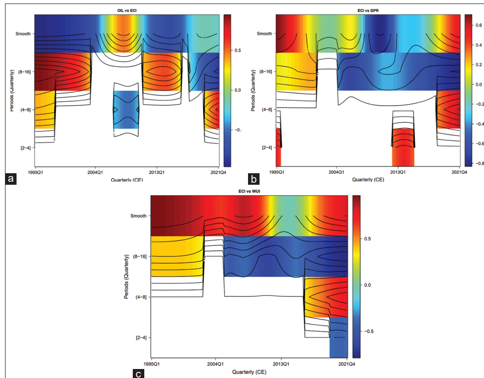
Figure 5: The WLMC heat-maps: The bivariate scenario GPR, WUI, and Oil vol. versus ECI. (a) Oil versus ECI, (b) GPR versus ECI, (c) WUI versus ECI
