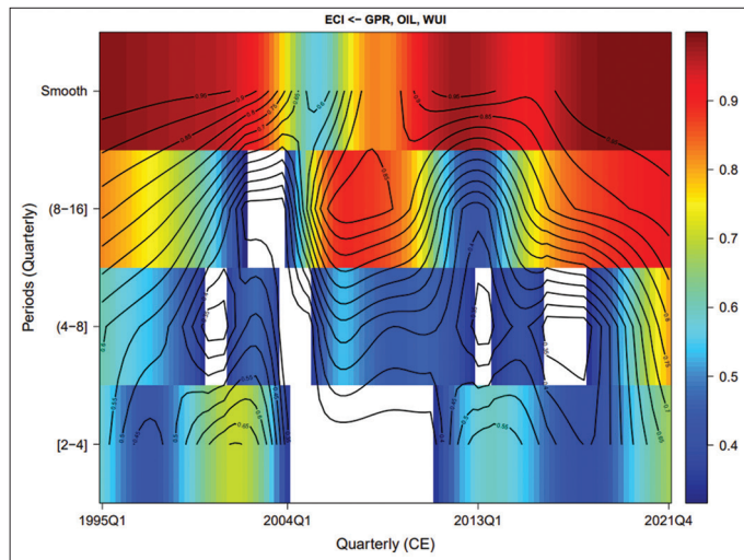
Figure 7: The WLMC heat-map for the four-variate case: Oil vol., GPR, WUI versus ECI
