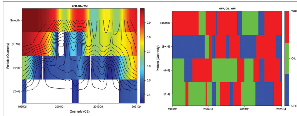
Figure 4: WLMC heat-map for the tri-variate scenario GPR, Oil vol., and WUI
