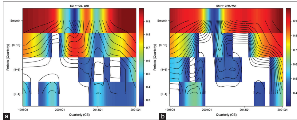
Figure 6: WLMC heat map for the tri-variate scenarios. (a) WLMC: Oil vol., WUI versus ECI, (b) WLMC: GPR, WUI versus ECI
