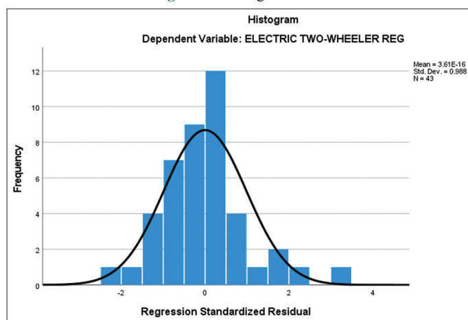
Figure 4: Histogram chart
