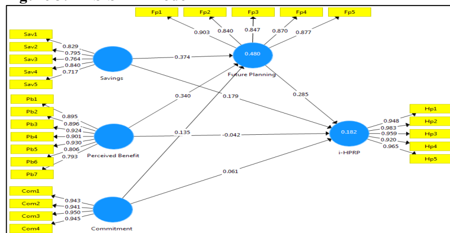
Figure 3: PLS-SEM Model
