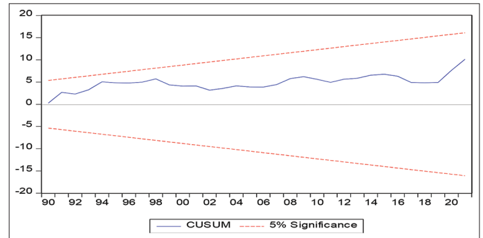
Figure 1: CUSUM test
