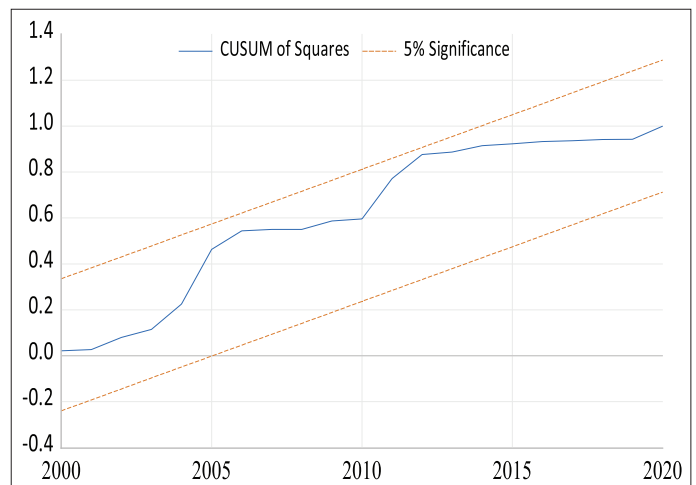
Figure 2: Plot of cumulative sum (CUSUM) of squares of recursive residuals
