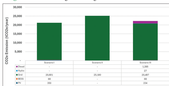
Figure 3: The result of greenhouse gas emissions in each scenario
