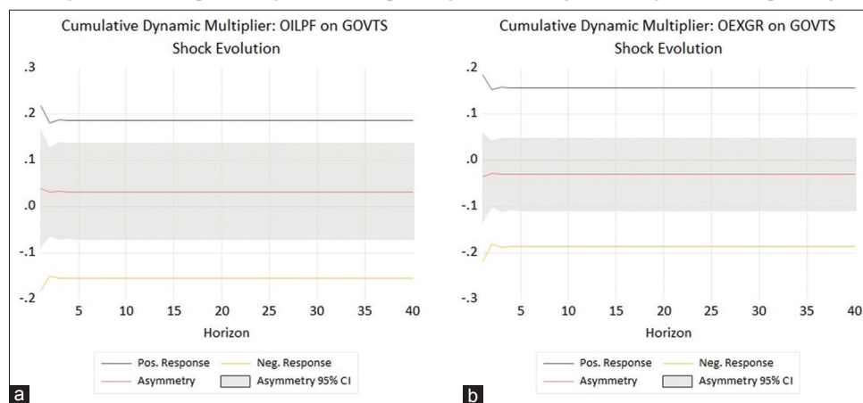
Figure 5: (a) Oil price on government spending. (b) Exchange rate on government spending
