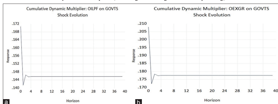
Figure 3: (a) auto-regressive distributed lag (ARDL) cumulative dynamic multiplier (oil price on government spending). (b) ARDL cumulative dynamic multiplier (exchange rate on government spending)
