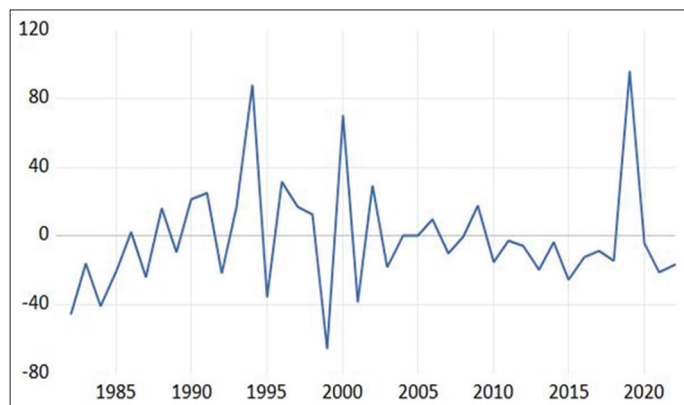
Figure 4: N-auto-regressive distributed lag cointegrating series
