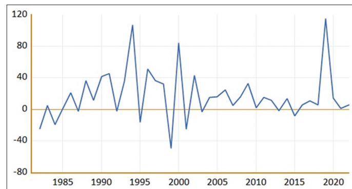
Figure 2: Auto-regressive distributed lag cointegrating series
