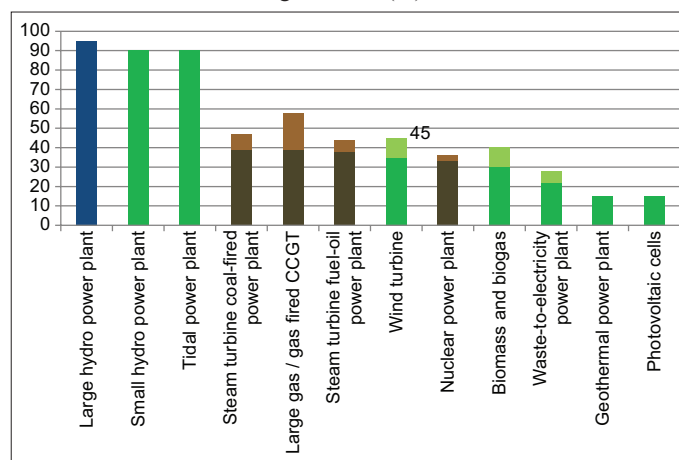
Graph 2: Efficiency of different technologies in electricity generation (%)
