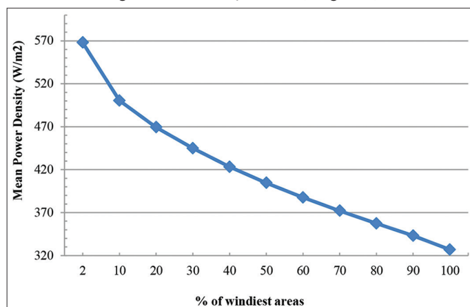
Figure 8: The mean power density for the 10% windiest areas in the selected region 500W/m 2 . Qafë Thane, Pogradec, Albania
