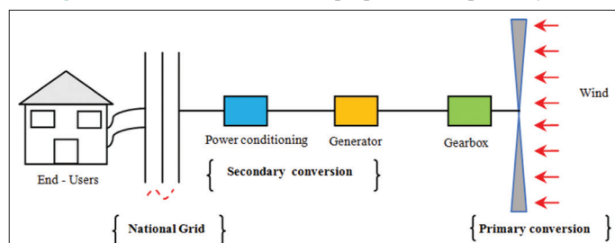
Figure 10: Schematisation of the proposed wind power system
