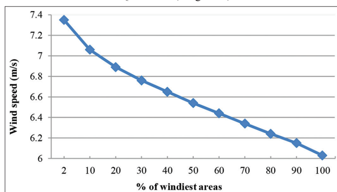
Figure 7: Wind speed variation at the proposed wind power plant location. Qafë-Thane, Pogradec, Albania
