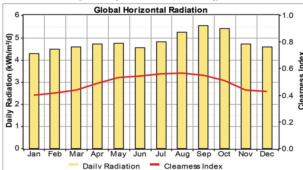
Figure 1: The potential of solar radiation in Yogyakarta
